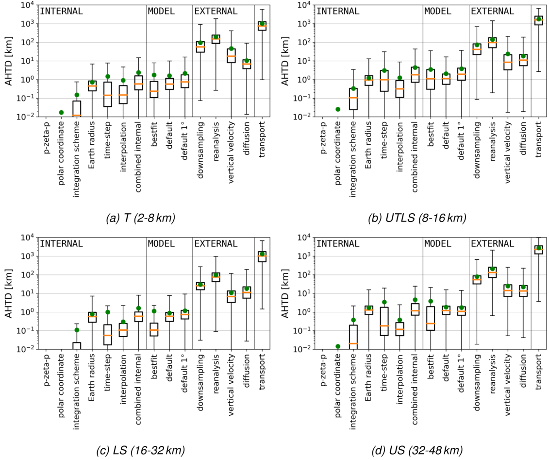
Figure 5.4: Horizontal deviations quantified with the AHTDs after 1 day forward calculation for the entire ensemble of air parcels splitted in four height layers. The boxplots indicate quartiles as defined in Fig. 5.2.
