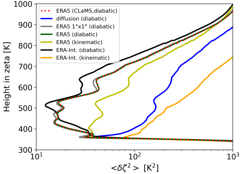
Figure 5.11: Profiles of the zeta variance \langle \delta \zeta^2 \rangle after 10 days as a measure of the cross-isentropic dispersion. All scenarios are calculated with MPTRAC, except “ERA5 (CLaMS,diabatic)”. The profiles for the scenarios “ERA5 (diabatic)” and “ERA5 (CLaMS,diabatic)” overlap each other. For the definition of the MPTRAC scenarios see also Table 5.1, from label “MPTRAC-default” to label “MPTRAC-def-erai-kin”.
