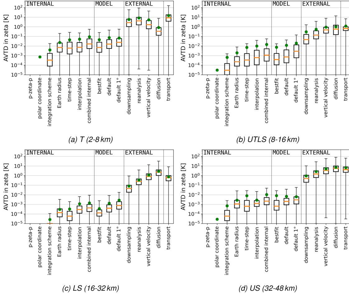
Figure 5.2: Different AVTDs in zeta coordinates after 1 day forward calculations for the entire ensemble of air parcels splitted into four height layers. The different uncertainty sources are defined in Table 5.2. The box plots show the median, quartiles (25% and 75%), minimum and maximum (outliers have been ignored if they are 10 times the inter-quartile difference). Green dots indicate the mean AVTDs. Deviations for the p-zeta-p transformation and the polar coordinate are lower than 10^{-5} K and do not show up here. The distinction between internal, model and external uncertainty sources is indicated by vertical lines.
